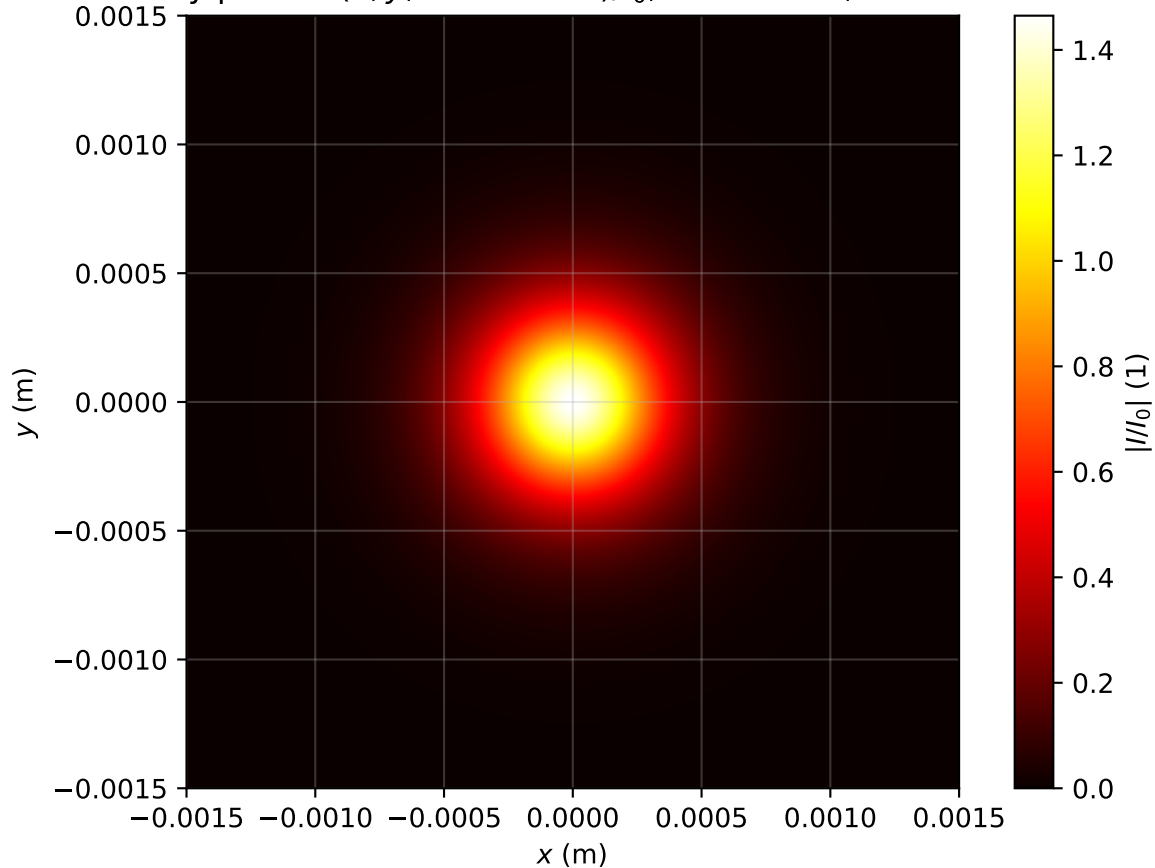
Intensity profile I(x, y, z = 3.662m)/I_0 , Pin=0.9Pcr, artificial time
